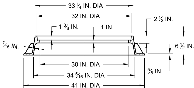
SECTION A-A FRAME
